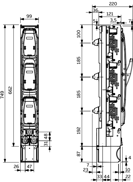
ZLBM2-3P-Z-M12 (1SEB000439)
