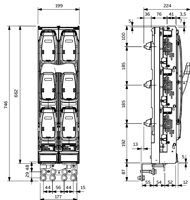
ZLBM800A-3P-Z-M12 (1SEB000443)
