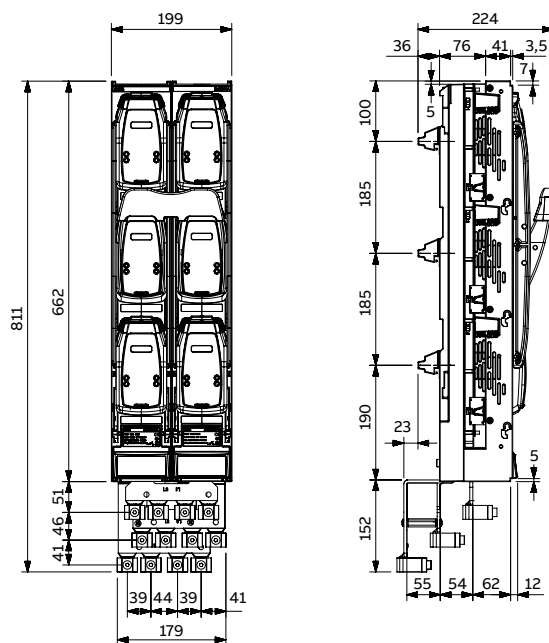
ZLBM800A-3P-Z-V (1SEB000444)
