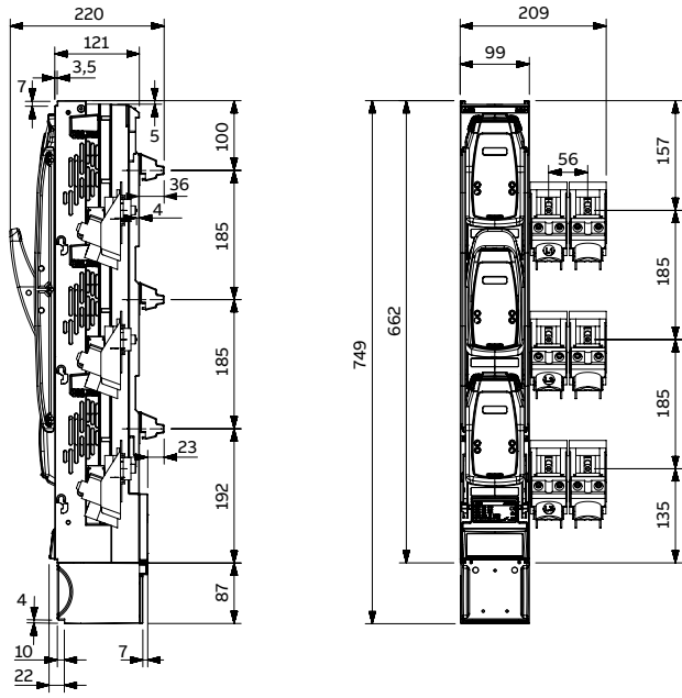
ZLBM3-3P-Z-2SC (1SEB000442)
