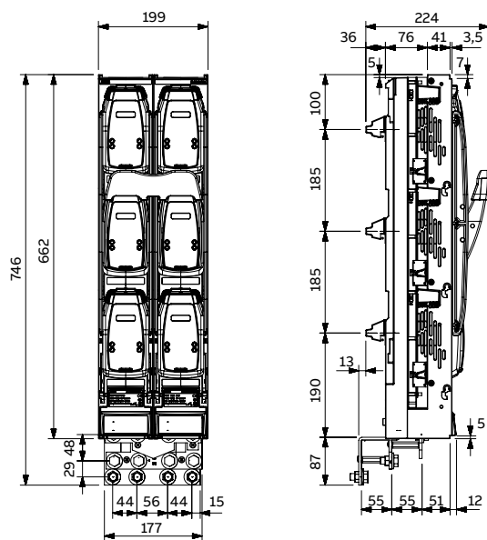
ZLBM800A-3P-Z-M12 (1SEB000443)
