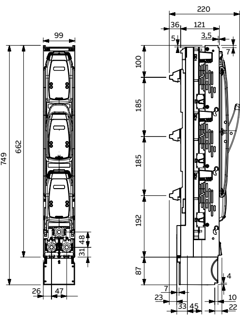
ZLBM3-3P-Z-M12 (1SEB000440)
